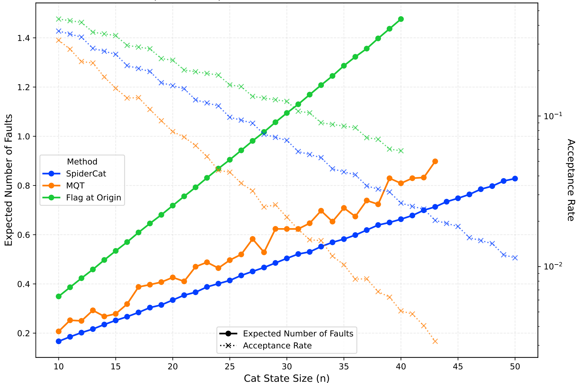
Method Comparison: Expected Number of Faults vs CAT state size (t=3)
