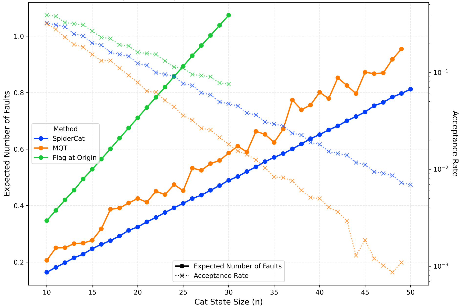
Method Comparison: Expected Number of Faults vs CAT state size (t=4)
