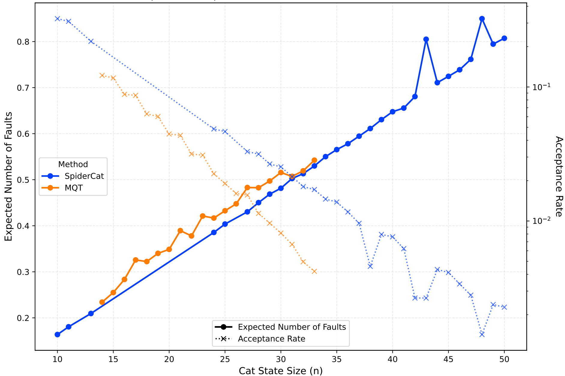
Method Comparison: Expected Number of Faults vs CAT state size (t=7)
