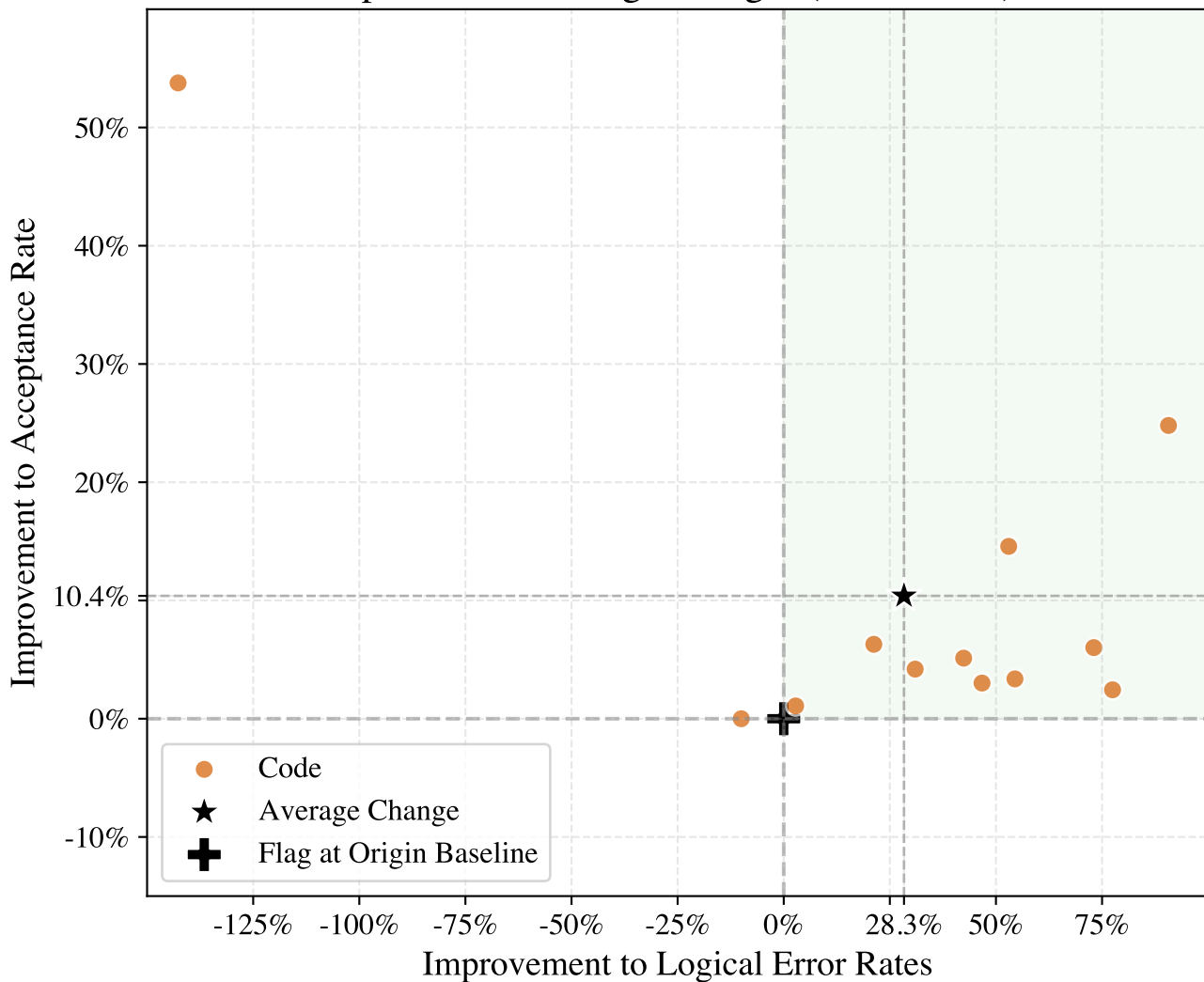
SpiderCSS vs Flag at Origin (LER & AR)
