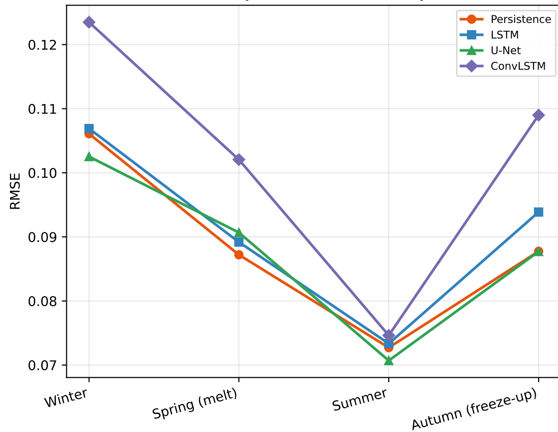
RMSE by season (lead = 7 days)
