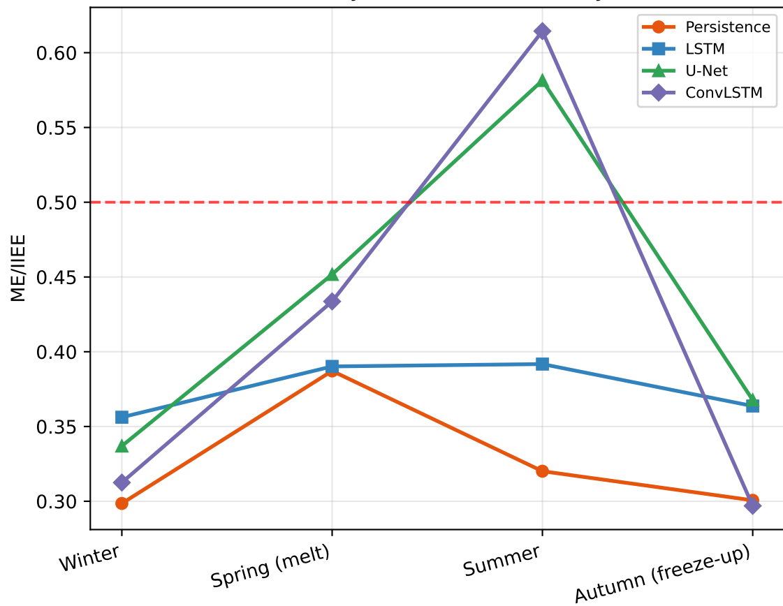
ME/IEE by season (lead = 7 days)
