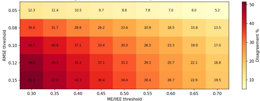
Metric Disagreement Rate (%) — Sensitivity to Threshold Choice
