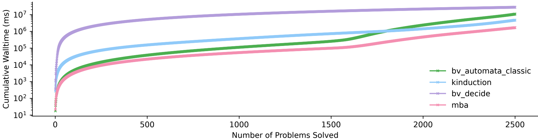
Number of Problems Solved vs Cumulative Walltime for Each Solver
