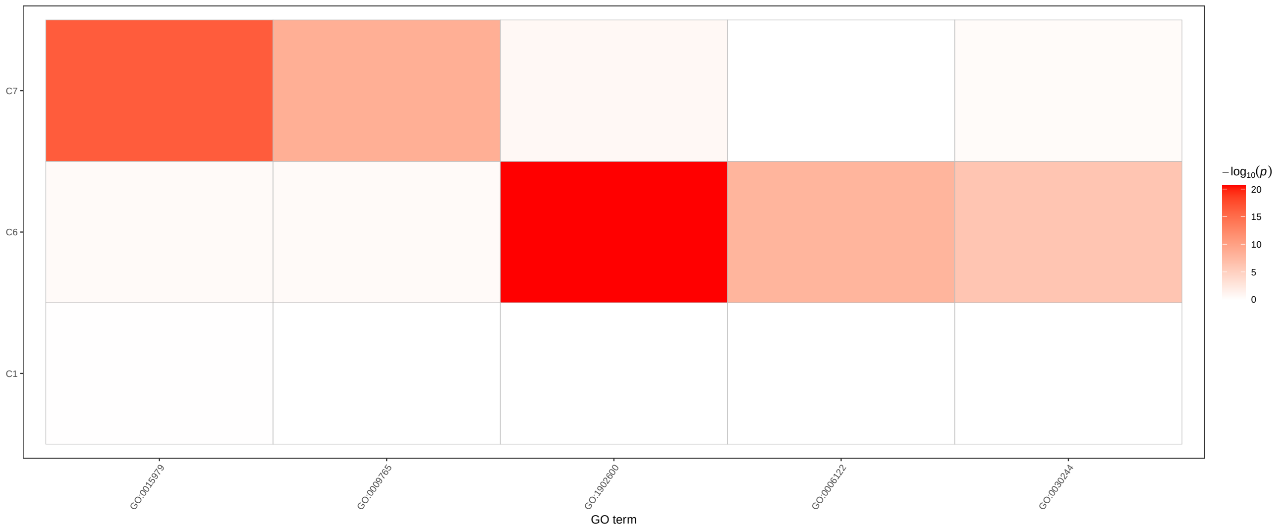
GO enrichment across clusters
