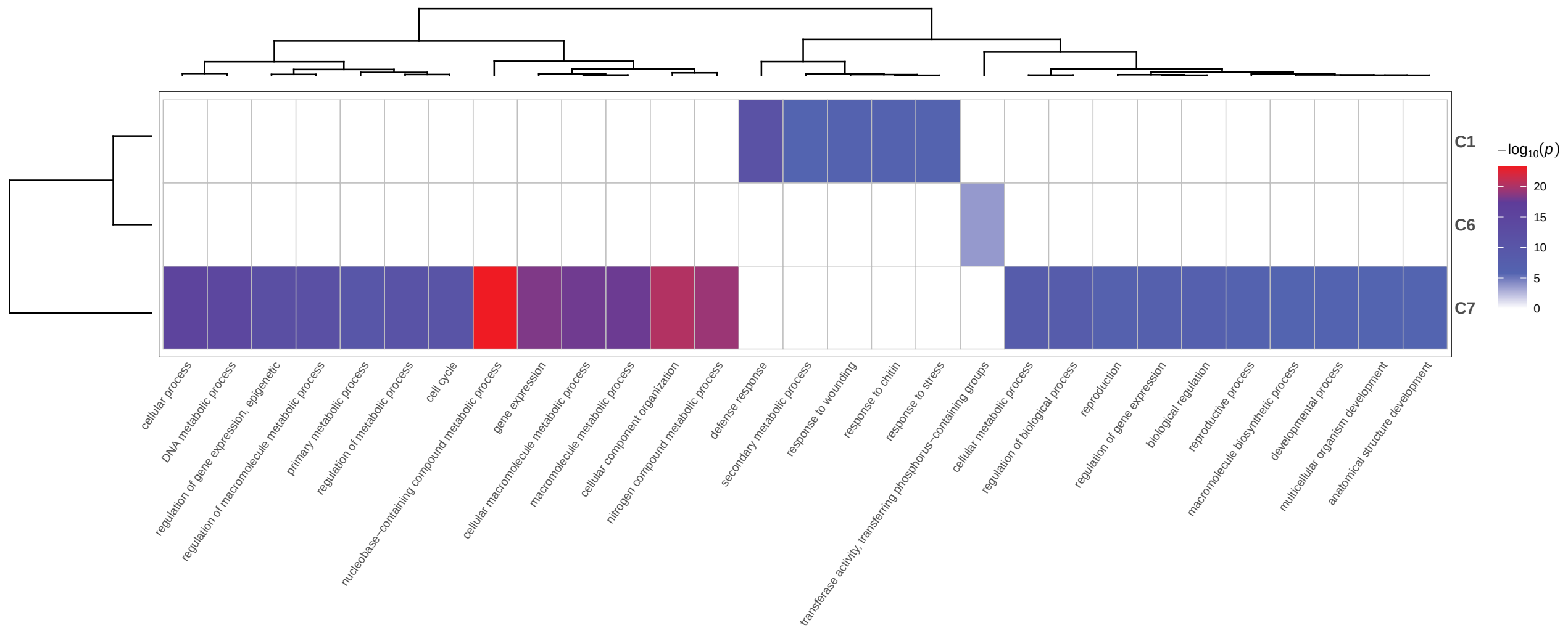
GO enrichment heatmap across clusters
