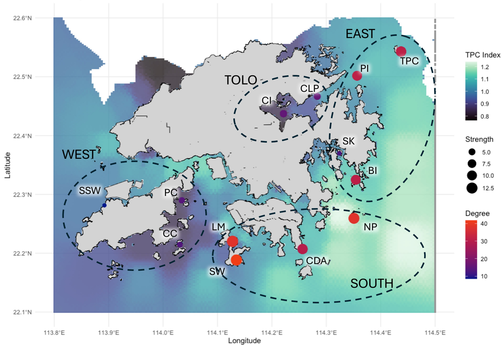
Figure 1: Locations of all 13 sampling sites. Strength and degree were the mean value of all temporal replications. Dotted line outlined the four regions. The background water gradient indicated TPC index modeled with mean Chlorophyll- a value between May 2017 – Dec 2022. Since TPC index is linearly modeled by Chlorophyll- a concentration, TPC gradient matched Chlorophyll- a gradient.
