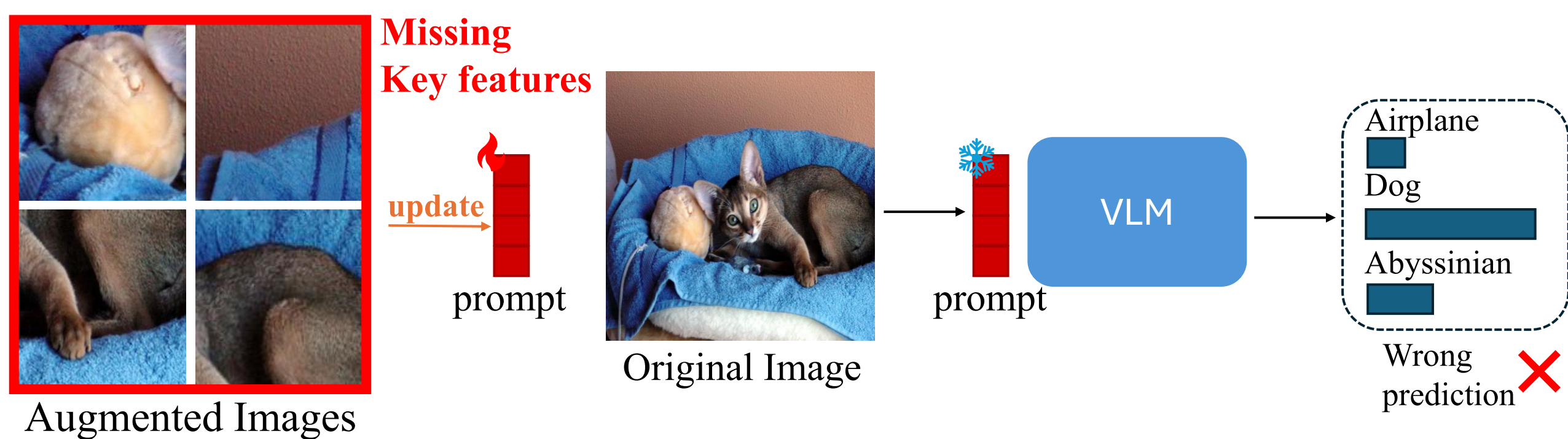
(a) Misguided Adaptation with Noisy Views
