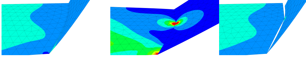
FIGURE 8. Zoom towards discrete crease lines for the folding and bending experiments corresponding to the full deformations shown in Figure ?? with crease line approximations (S1), (S2), and (S3) (from left to right) and geometric refinements towards the entire crease line in case of (S1) and towards the corner points in case of (S2) and (S3).
