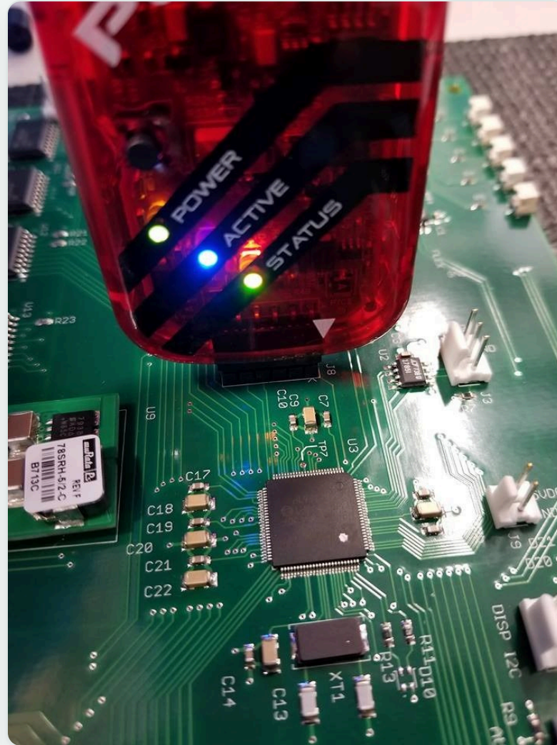
Firmware updates: programmer connected to a circuit board
