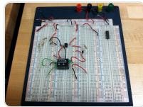
Breadboard
