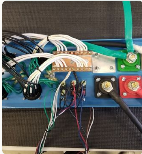
Chassis with heavy power lugs and busbar
