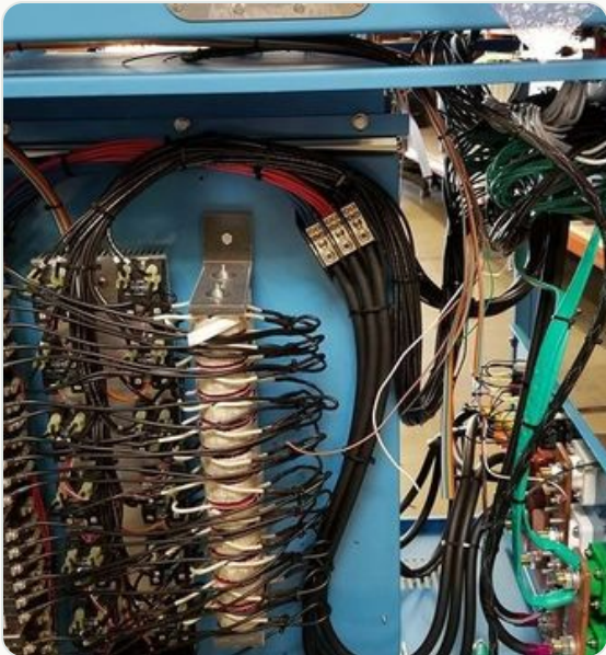
Wired and assembled: control cabinet
