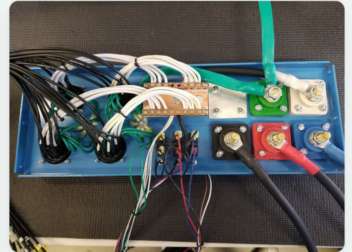
Chassis with heavy power lugs and busbar
