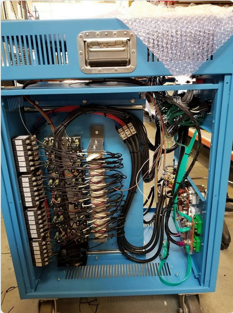
Wired and assembled: control cabinet
