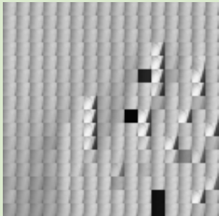
SELF-ATTENTION OUTPUT
