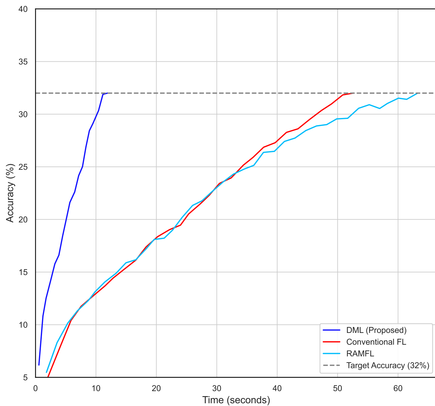
(a) CIFAR-100 dataset (IID data)
