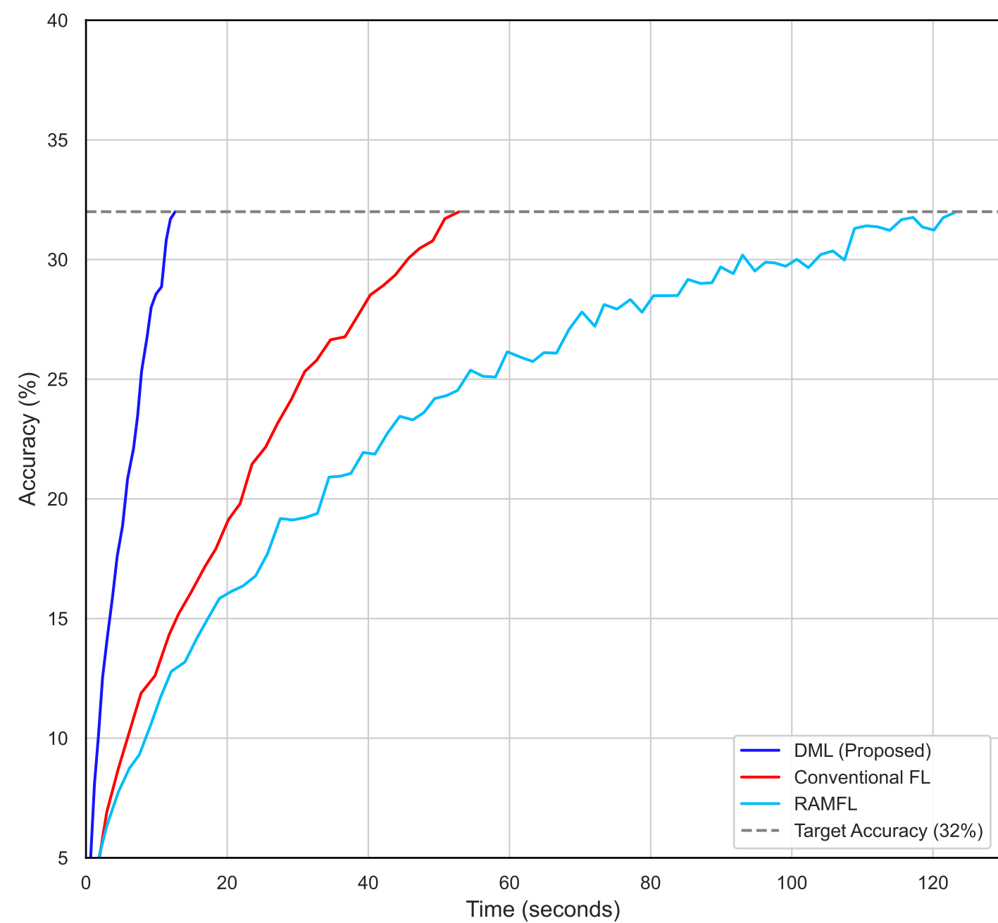
(b) CIFAR-100 dataset (non-IID data)
