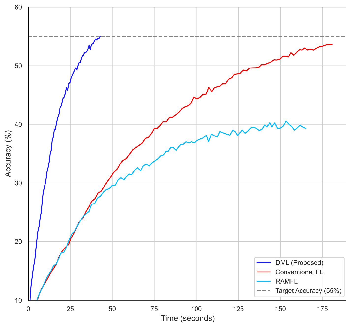
(a) CIFAR-10 dataset (IID data)
