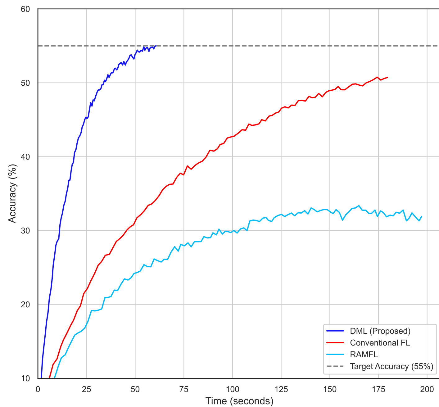
(b) CIFAR-10 dataset (non-IID data)
