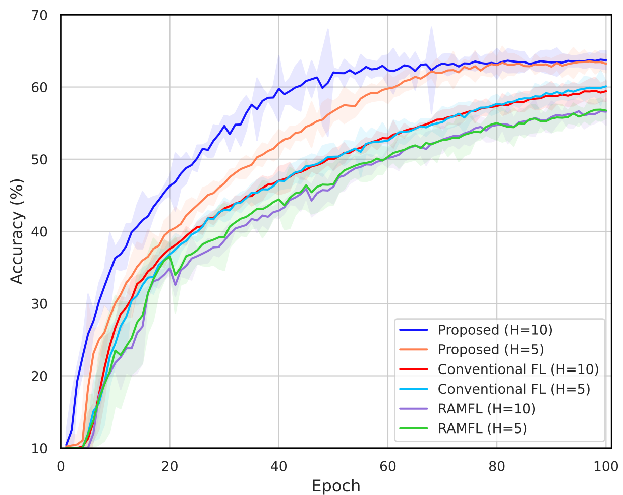
(b) CIFAR-10 dataset (non-IID data)
