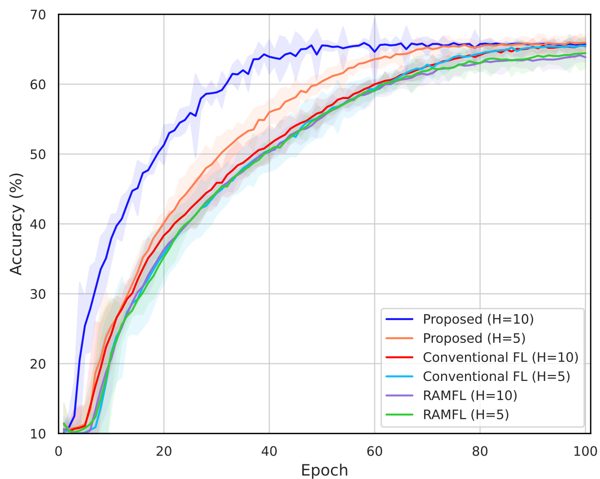
(a) CIFAR-10 dataset (IID data)
