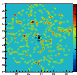
ResidualSig 158.49TeV&lt;E&lt;251.19TeV
