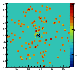
ResidualSig 251.19TeV&lt;E&lt;398.11TeV
