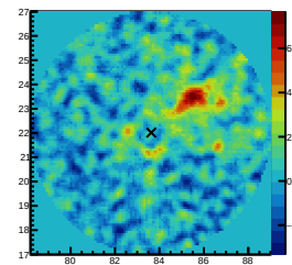
ResidualSig 63.10TeV&lt;E&lt;100.00TeV
