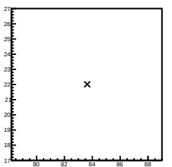
ResidualSig 1584.89TeV&lt;E&lt;2511.89TeV
