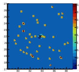
ResidualSig 398.11TeV&lt;E&lt;630.96TeV
