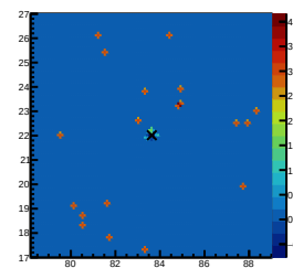
ResidualSig 630.96TeV&lt;E&lt;1000.00TeV
