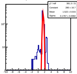
ResidualSig1D 251.19TeV&lt;E&lt;398.11TeV
