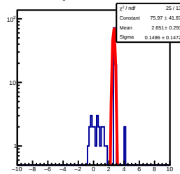
ResidualSig1D 630.96TeV&lt;E&lt;1000.00TeV
