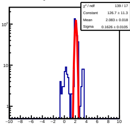
ResidualSig1D 398.11TeV&lt;E&lt;630.96TeV
