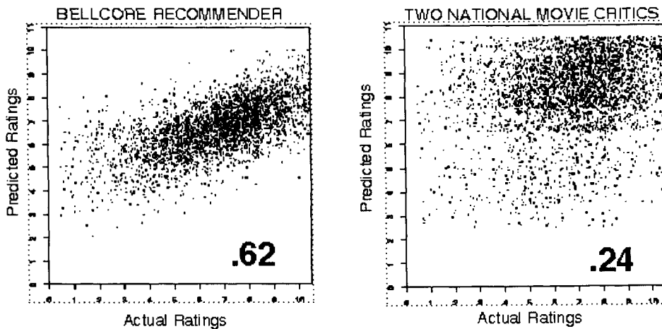
Figure 7. Video recommender scatterplots.
