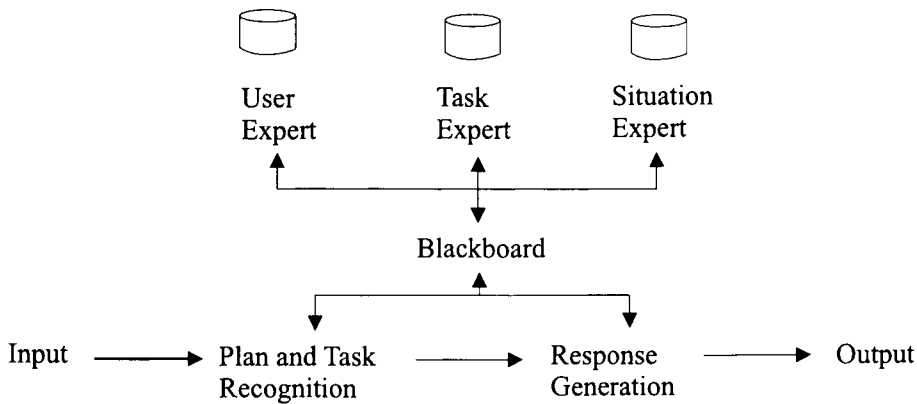
Figure 4. Typical components of a blackboard system.
