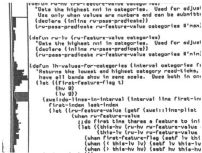
Figure 16. Attributed-Mapped Scroll Bar. The scroll bar depicts a graphical summary of the history of editing this code.
