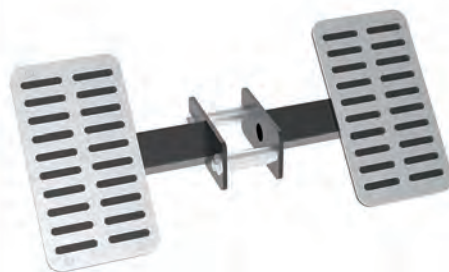
RA26 Low Row Foot Plate Attachment
