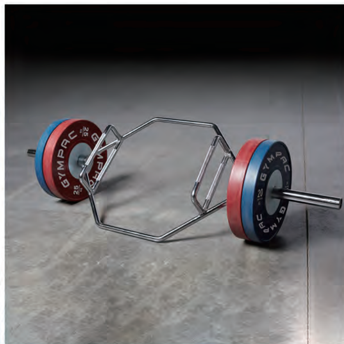
SB08-56 Olympic Hex Trap bar Total length: 56" Grip diameter: 28 mm Bar weight: 24 kg SB08-63 Olympic Hex Trap bar Total length: 63" Grip diameter: 28 mm Bar weight: 27 kg SB08-71 Olympic Hex Trap bar Total length: 71" Grip diameter: 28 mm Bar weight: 31 kg
