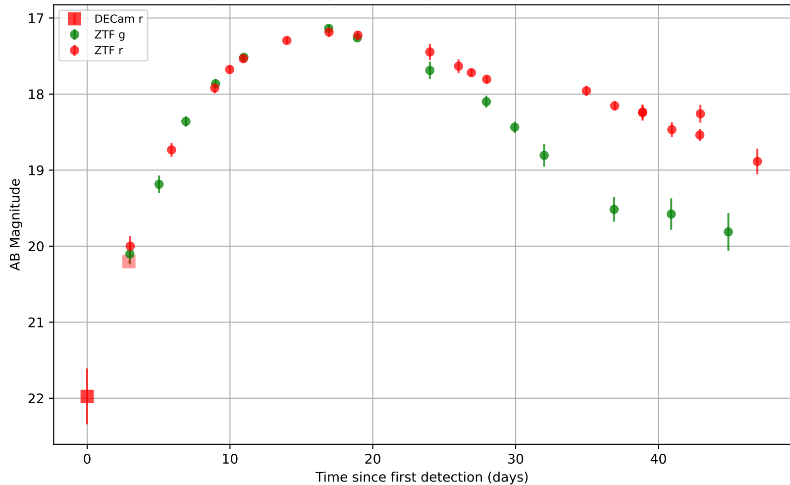
Photometry of SN2025kwy (ZTF25aaqsuda, C202505201402422m202612)
