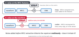
Two ways to train for noise
