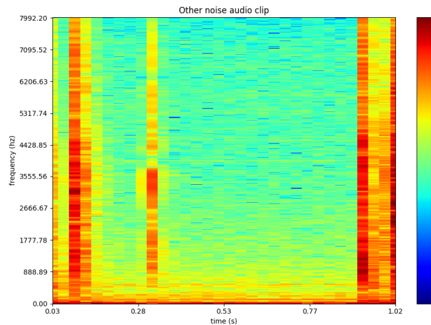
Fig. 2. Example of other noise in spectrogram representation
