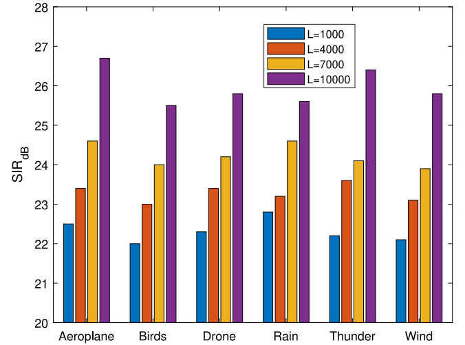
Fig. 8. SIR performance of the FastICA algorithm for different data block lengths.
