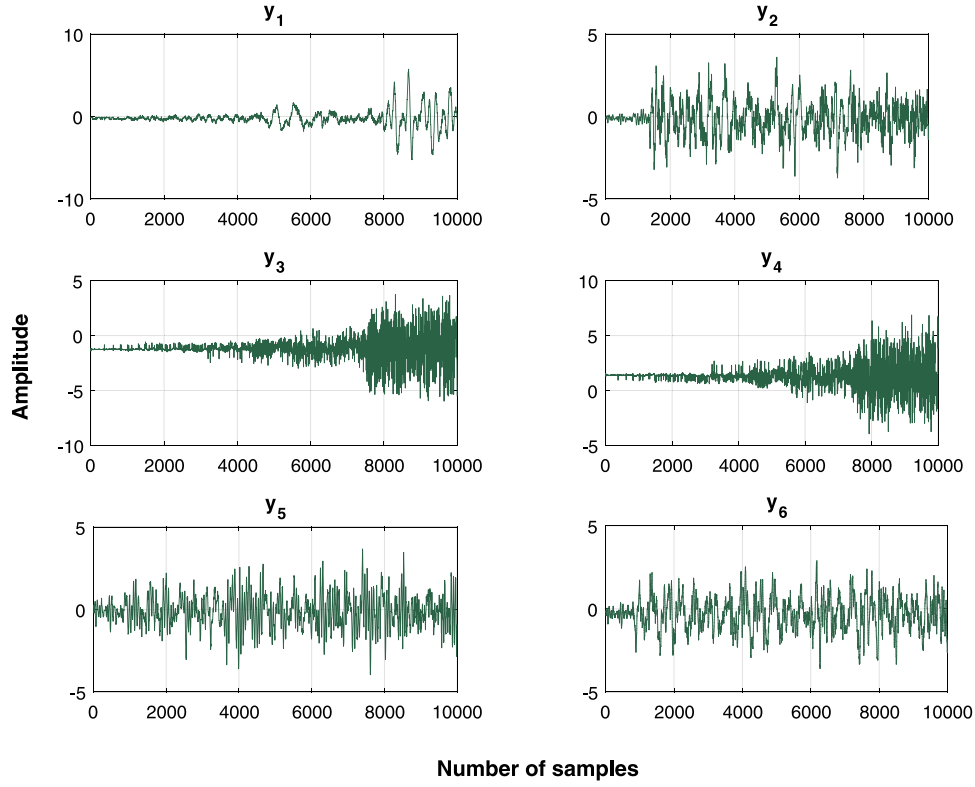
Fig. 7. ICA estimated audio source signals through FastICA algorithm.
