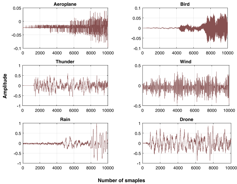
Fig. 3. Audio source signals of the aeroplane, bird, wind, rain, thunder, and the AmDr recorded through microphone.
