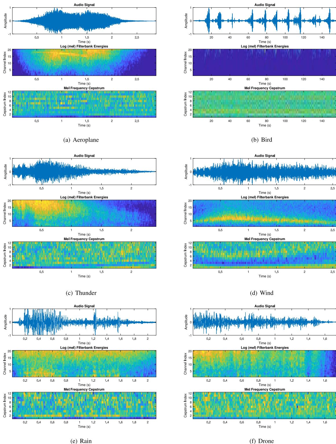
Fig. 10. MFCC of different audio signals.
