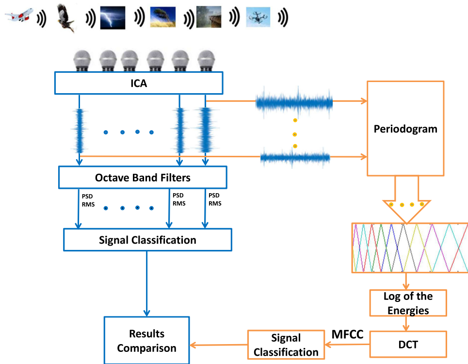
Fig. 6. Block diagram representation of the proposed drone detection technique.
