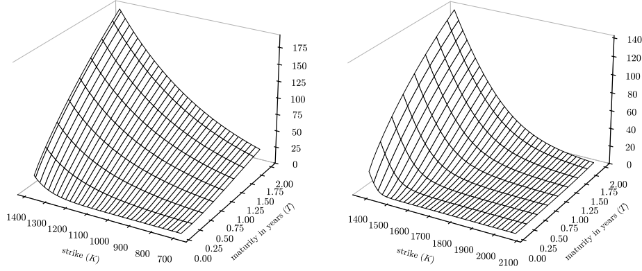
FIGURE 1. Heston OTM option prices for S_{\text{ref}} 1383.8158 on April 20, 2012 with \Phi^* = (0.1181, 1.3381, 1.1057, -0.7922, 0.0275) : puts wing (left) and calls wing (right).
