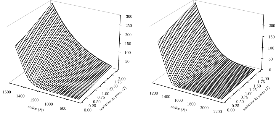
FIGURE 1. Heston option prices for S_{\text{ref}} 1358.1765 on May 11, 2012 with \Phi^* = (0.1302, 1.0255, 1.0582, -0.7401, 0.034) : puts wing (left) and calls wing (right).
