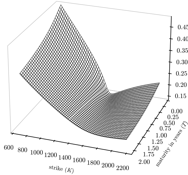
FIGURE 2. Out of the money implied volatilities from Figure 3
