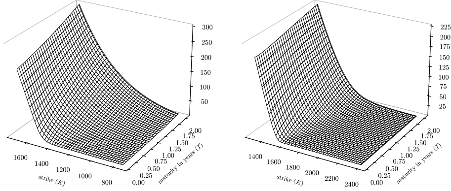
FIGURE 3. Bates option prices for S_{\text{ref}} = 1500.3753 on January 25, 2013 with \Theta^* = (0.0614, 0.5533, 0.3767, -0.763, 0.0103, 0.0724, -0.2699, 0.3294) : puts wing (left) and calls wing (right).
