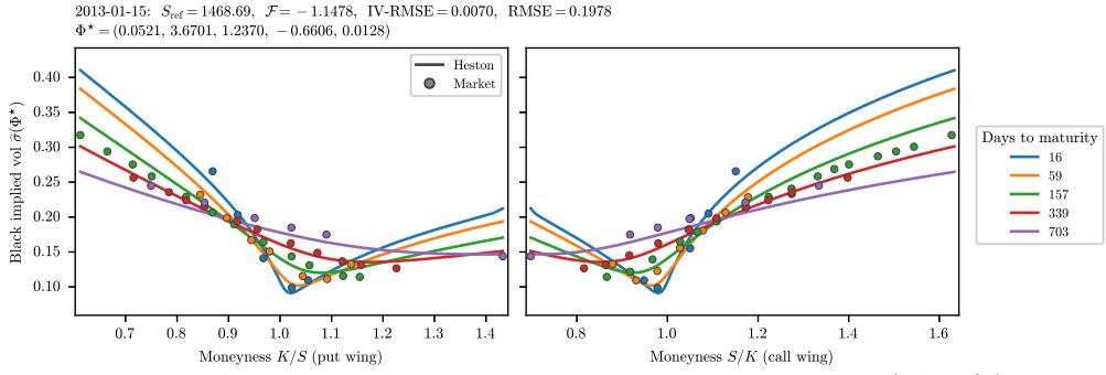
FIGURE 10. Heston implied-volatility smiles for January 15, 2013: put wing (left, K/S ) and call wing (right, S/K ), with market trades scattered.
