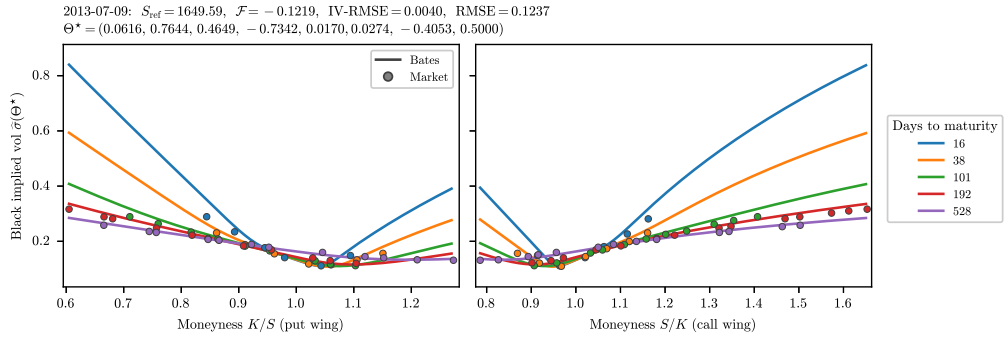
FIGURE 18. Bates implied-volatility smiles for July 09, 2013: put wing (left, K/S ) and call wing (right, S/K ), with market trades scattered.
