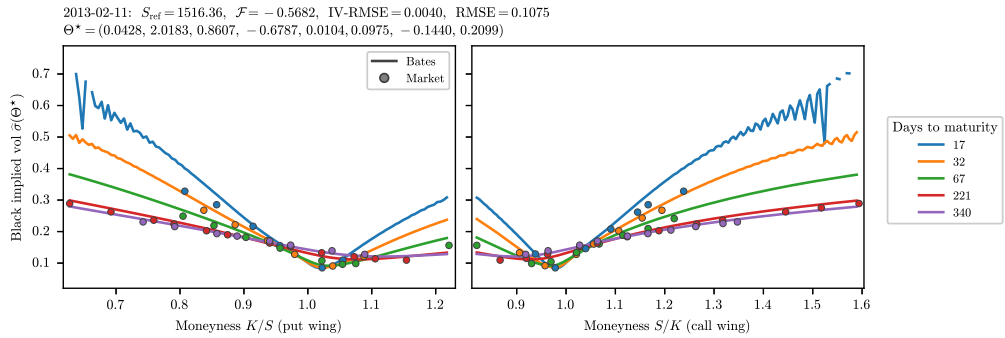
FIGURE 20. Bates implied-volatility smiles for February 11, 2013: put wing (left, K/S ) and call wing (right, S/K ), with market trades scattered.
