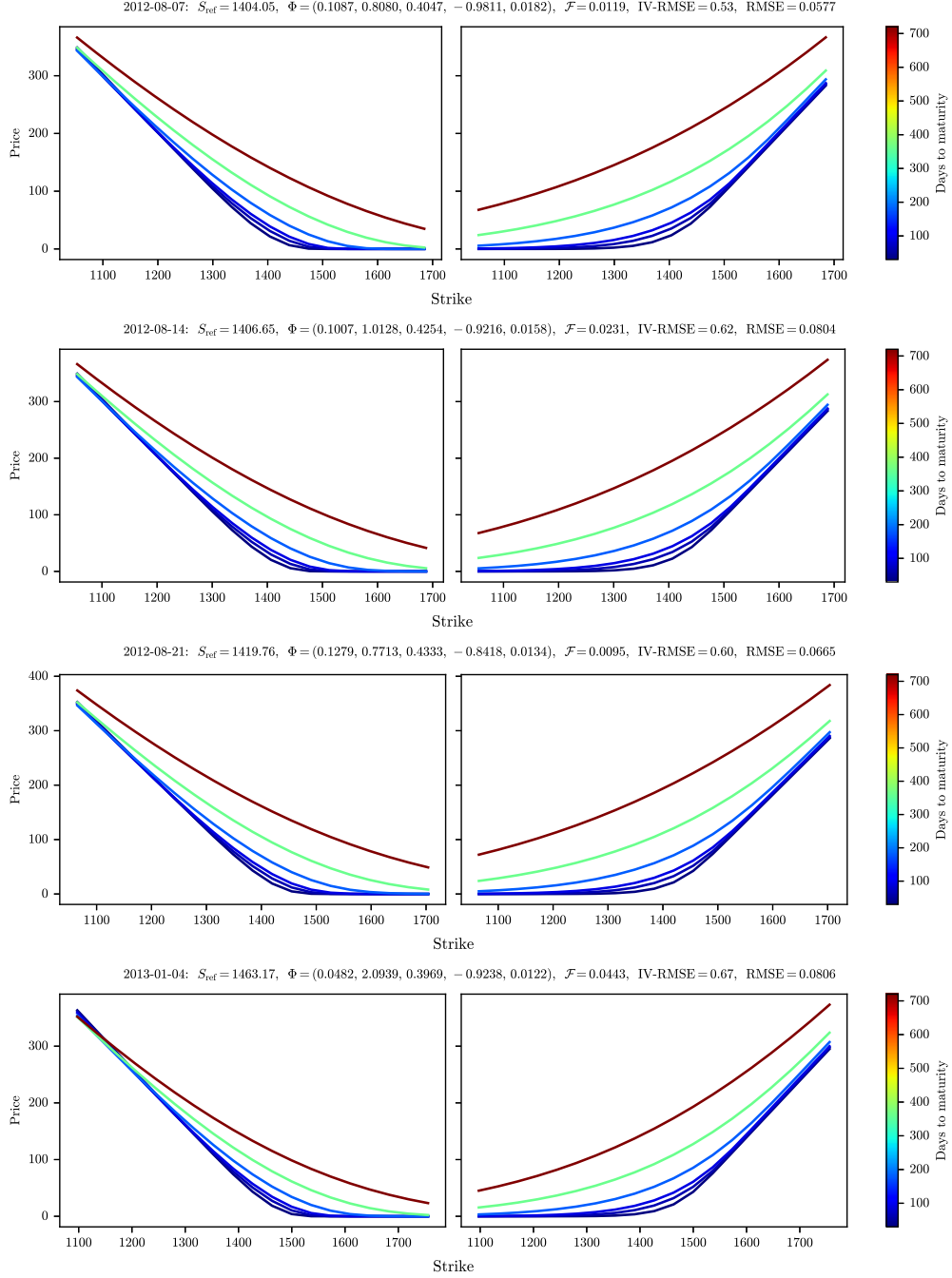
FIGURE 3. Heston option prices for August 07, 2012, August 14, 2012, August 21, 2012, January 04, 2013: put wing (left) and call wing (right) per day.
