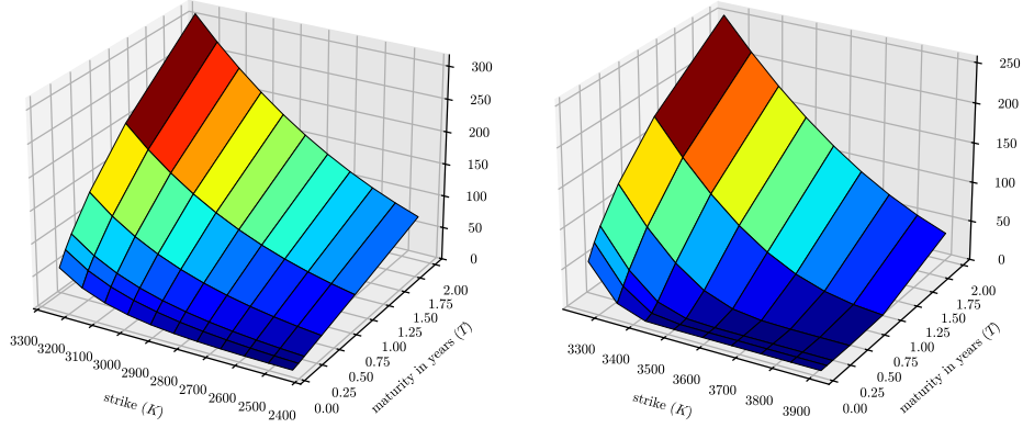
FIGURE 1. Heston OTM option prices for S_{\text{ref}} = 3254.0554 on March 16, 2020 with \Phi = (0.0313, 9.9238, 1.488, -0.9238, 0.0343) : puts wing (left) and calls wing (right).
