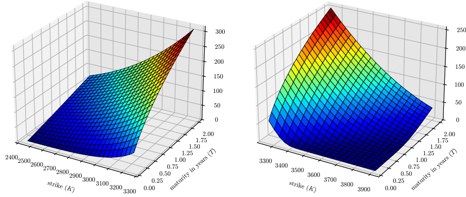
FIGURE 1. Heston OTM option prices for S_{\text{ref}} 3254.0554 on March 16, 2020: puts wing (left) and calls wing (right).
