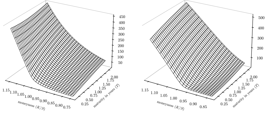
FIGURE 1. Heston option prices for S_{\text{ref}} = 2939.9736 on May 03, 2019 with \Phi^* = (0.043, 3.88, 1.7589, -0.6901, 0.013) : puts wing (left) and calls wing (right).
