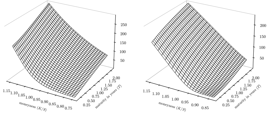
FIGURE 3. Bates option prices for S_{\text{ref}} = 1293.0412 on January 10, 2012 with \Theta^* = (0.0905, 0.8458, 0.5875, -0.8327, 0.0319, 0.0646, -0.5, 0.4875) : puts wing (left) and calls wing (right).
