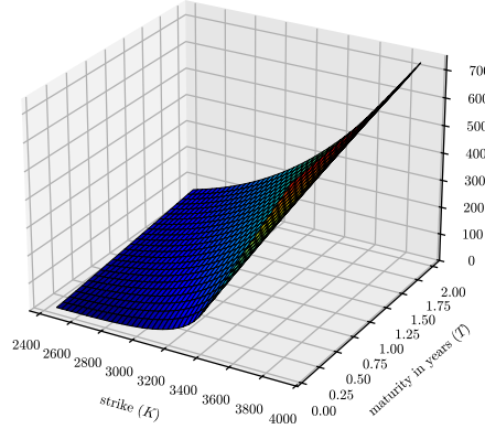
FIGURE 1. Heston OTM option prices for S_{\text{ref}} 3254.0554 on March 16, 2020 with \Phi = (0.0313, 9.9238, 1.488, -0.9238, 0.0343) : puts wing (left) and calls wing (right).
