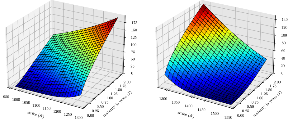
FIGURE 1. Heston OTM option prices for snapped S_{\text{ref}} 1280.2781 on January 03, 2012: puts wing (left) and calls wing (right).
