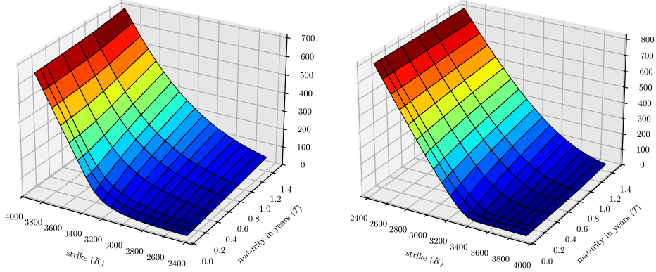
FIGURE 2. All put (left) and call (right) options from Figure 1
