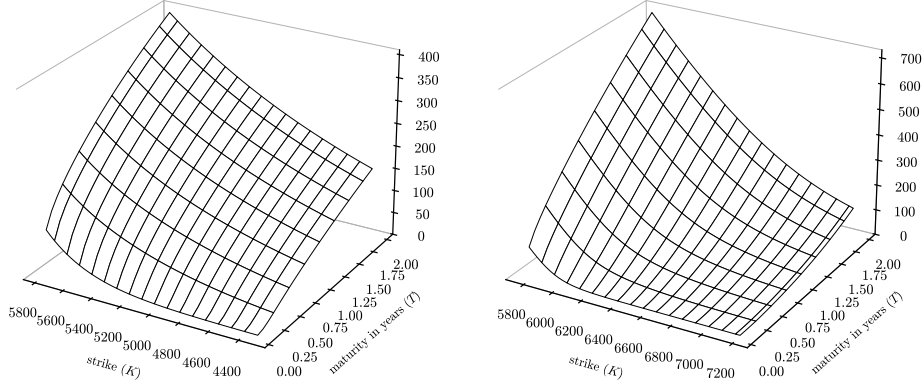
FIGURE 1. Heston OTM option prices for S_{\text{ref}} = 5777.2277 on October 10, 2024 with \Phi^* = (0.081, 0.768, 1.0023, -0.6986, 0.0322) : puts wing (left) and calls wing (right).
