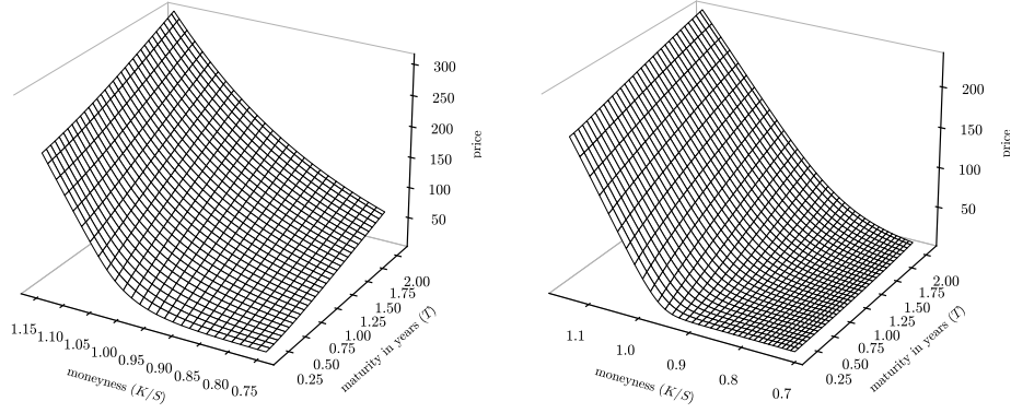
FIGURE 3. Bates option prices for S_{\text{ref}} = 1452.6941 on October 16, 2012 with \Theta^* = (0.1096, 0.4231, 0.4998, -0.7133, 0.0158, 0.0524, -0.3164, 0.3976) : puts wing (left) and calls wing (right).
