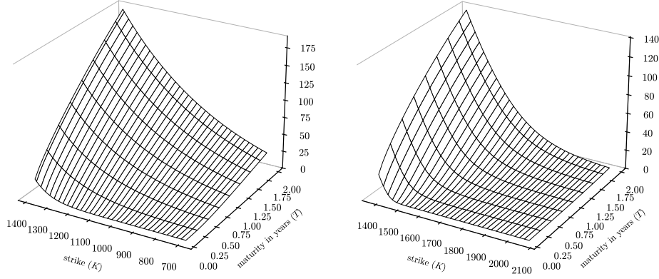
FIGURE 1. Heston OTM option prices for S_{\text{ref}} 1383.7348 on April 20, 2012 with \Phi^* = (0.1434, 0.8297, 0.9248, -0.8131, 0.0311) : puts wing (left) and calls wing (right).
