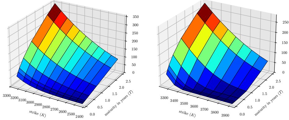
FIGURE 1. Heston OTM option prices for S_{\text{ref}} 3254.0554 on March 16, 2020 with \Phi = (0.0313, 9.9238, 1.488, -0.9238, 0.0343) : puts wing (left) and calls wing (right).
