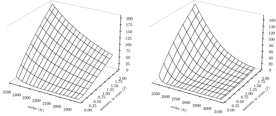
FIGURE 1. Heston OTM option prices for S_{\text{ref}} 2469.6922 on July 19, 2017 with \Phi^* = (0.0536, 1.2092, 0.7441, -0.8027, 0.0062) : puts wing (left) and calls wing (right).
