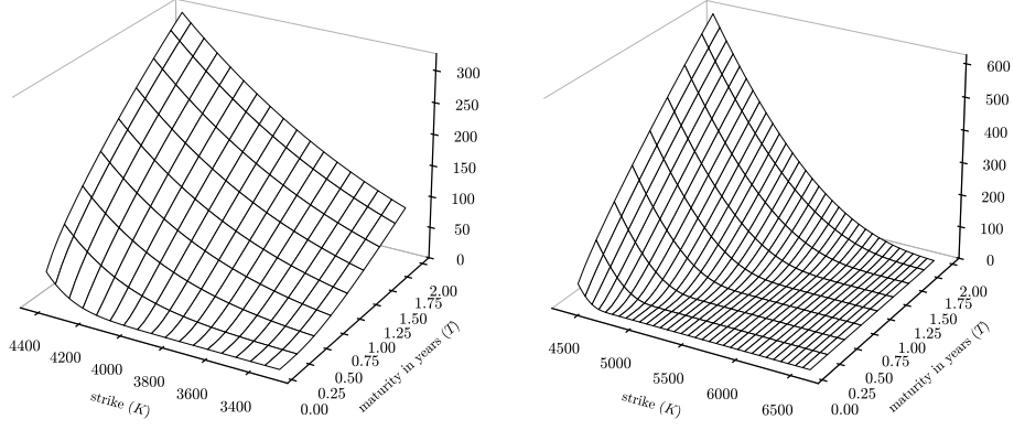
FIGURE 1. Heston OTM option prices for S_{\text{ref}} 4407.3262 on June 15, 2023 with \Phi^* = (0.2522, 0.1273, 0.2141, -0.9633, 0.0125) : puts wing (left) and calls wing (right).
