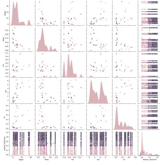
Figure 5: Joint distribution of Barrier Option prices and Heston [12] model parameters
