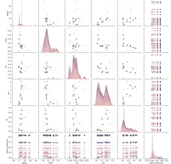
Figure 6: Joint distribution of Asian Option prices and Heston [8] model parameters
