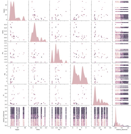
Figure 5: Joint distribution of Barrier Option prices and Heston [8] model parameters
