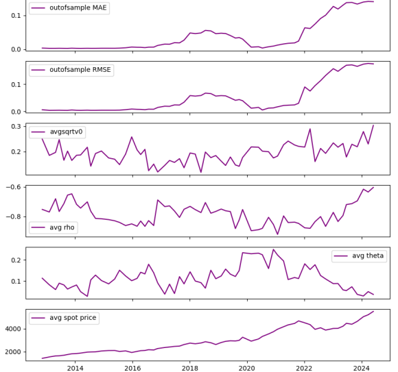
Figure 4: Out-of-sample average errors for Asian options
