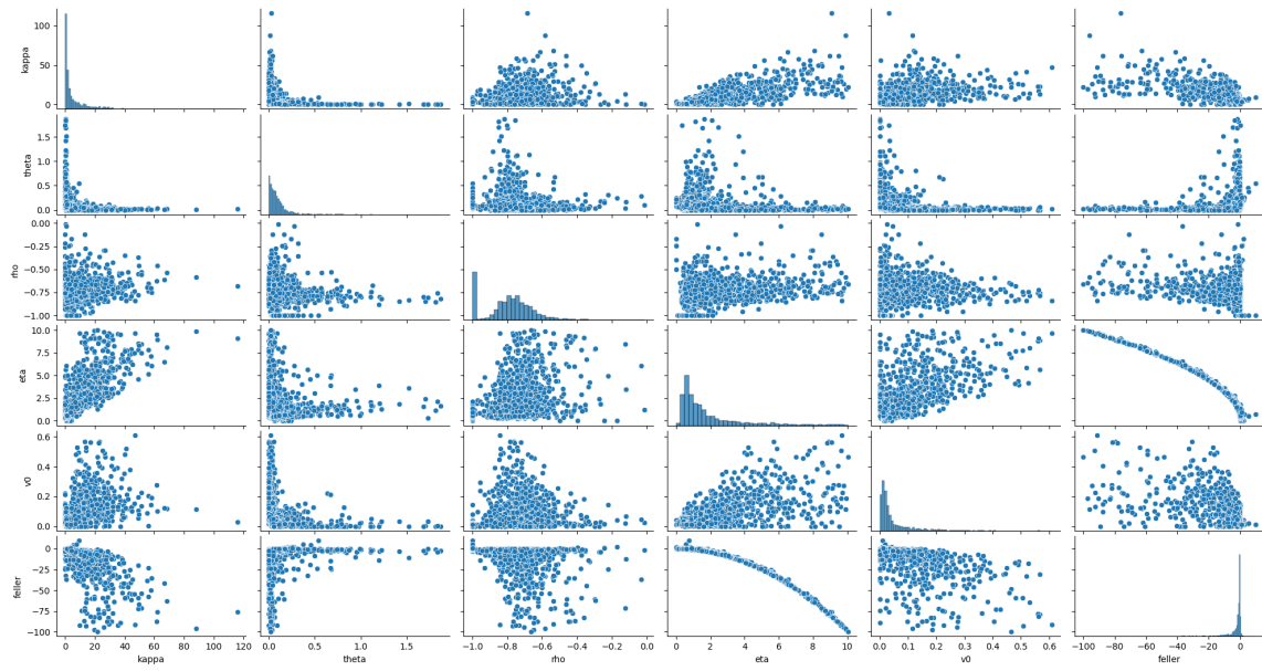
Figure 7: Distribution of Heston [13] pricing model parameters
