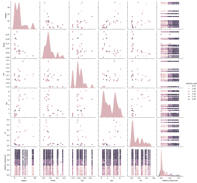
Figure 5: Shapely results of Barrier option testing
