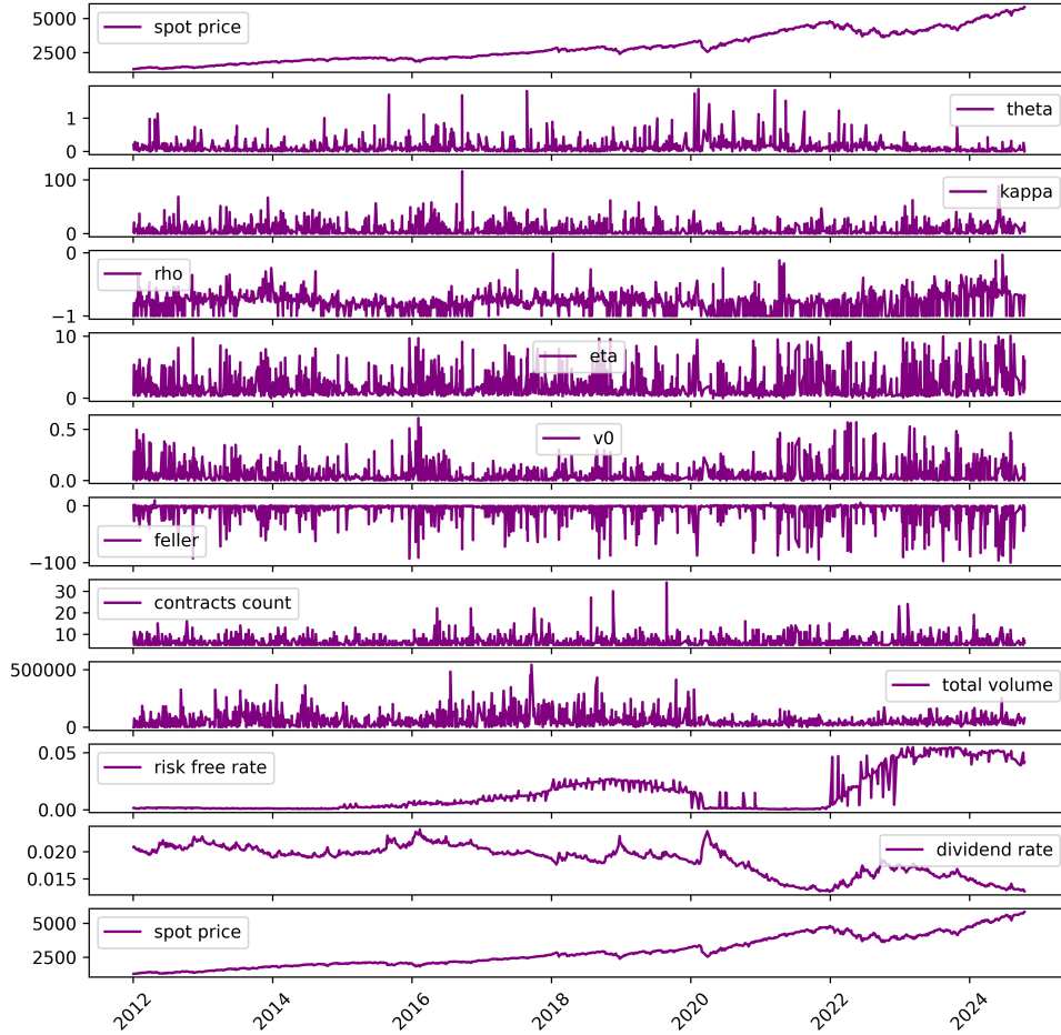
Figure 1: Plot of retrieved historical Heston [13] model parameters, underlying S , risk-free, and dividend rates for the SPX options market
