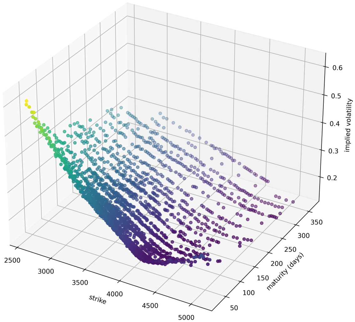
Figure 6: Illustrative set of implied volatilities extracted from one day of live Cboe SPX options trade data
