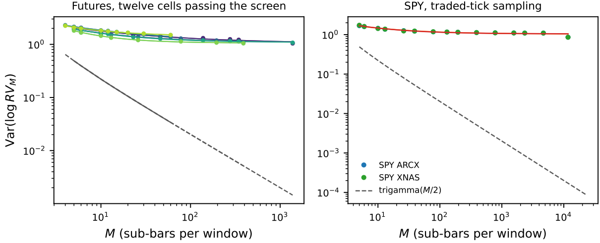
Figure 1: \text{Var}(\log RV_M) against M on log axes. Left: the twelve futures cells passing the tightened screen, points read from artifacts/s08-final/phase4_lambda.csv and fitted curves from artifacts/s10-exponent-audit/phase1_bootstrap.csv . Right: both SPY venues under traded-tick sampling, points from artifacts/s07-completion-and-spy/phase6_spy_grid_{ARCX,XNAS}.csv . Dashed lines are \text{trigamma}(M/2) on each grid. Twelve futures cells and two SPY venues pass the screen, fourteen in total; the twelve futures cells are six distinct cells under two boundary treatments that give identical fits.
