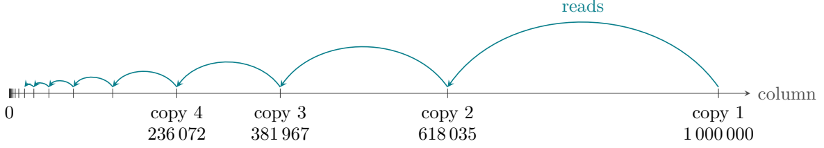
FIGURE 5. Where the copies work when the outermost copy reaches column N = 10^6 , with symbols passed one at a time. Each tick marks the next column of one copy. Each arc leads from where a copy writes to where it reads, which is where the next copy writes. The ticks crowd towards the left and end with the 22nd copy, before column 48.
