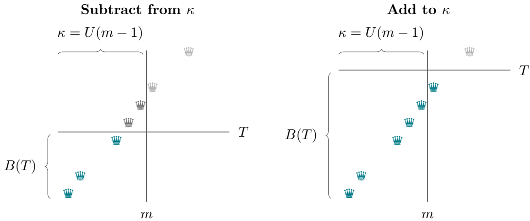
FIGURE 4. The adjustments in (19). Left: upper queens left of m and above T are subtracted from \kappa . Right: those right of m and at or below T are added. Upper-queen rows increase with their columns (Lemma 2), so at most one adjustment is nonzero. Teal queens are counted by B(T) .
