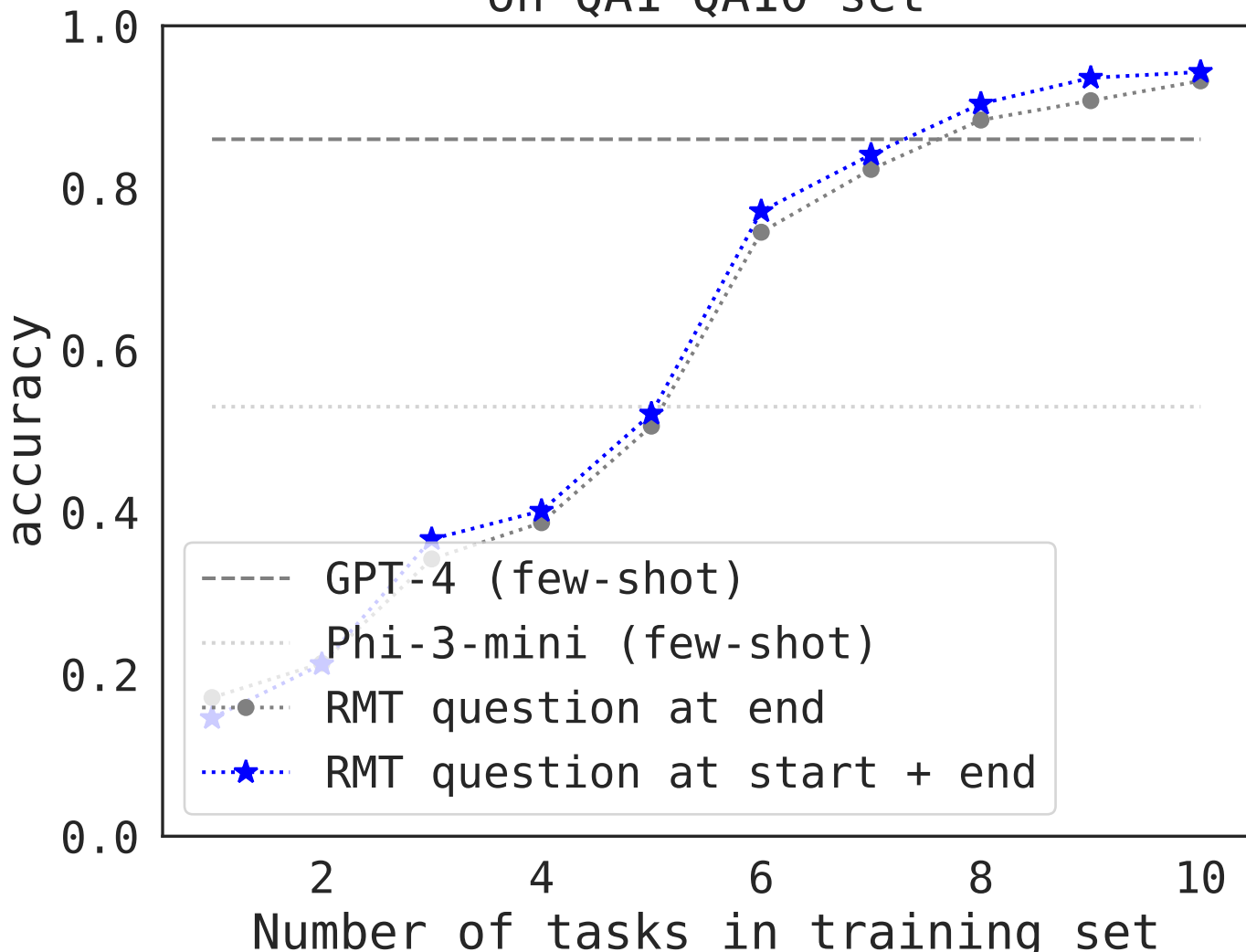
Average performance on QA1-QA10 set
