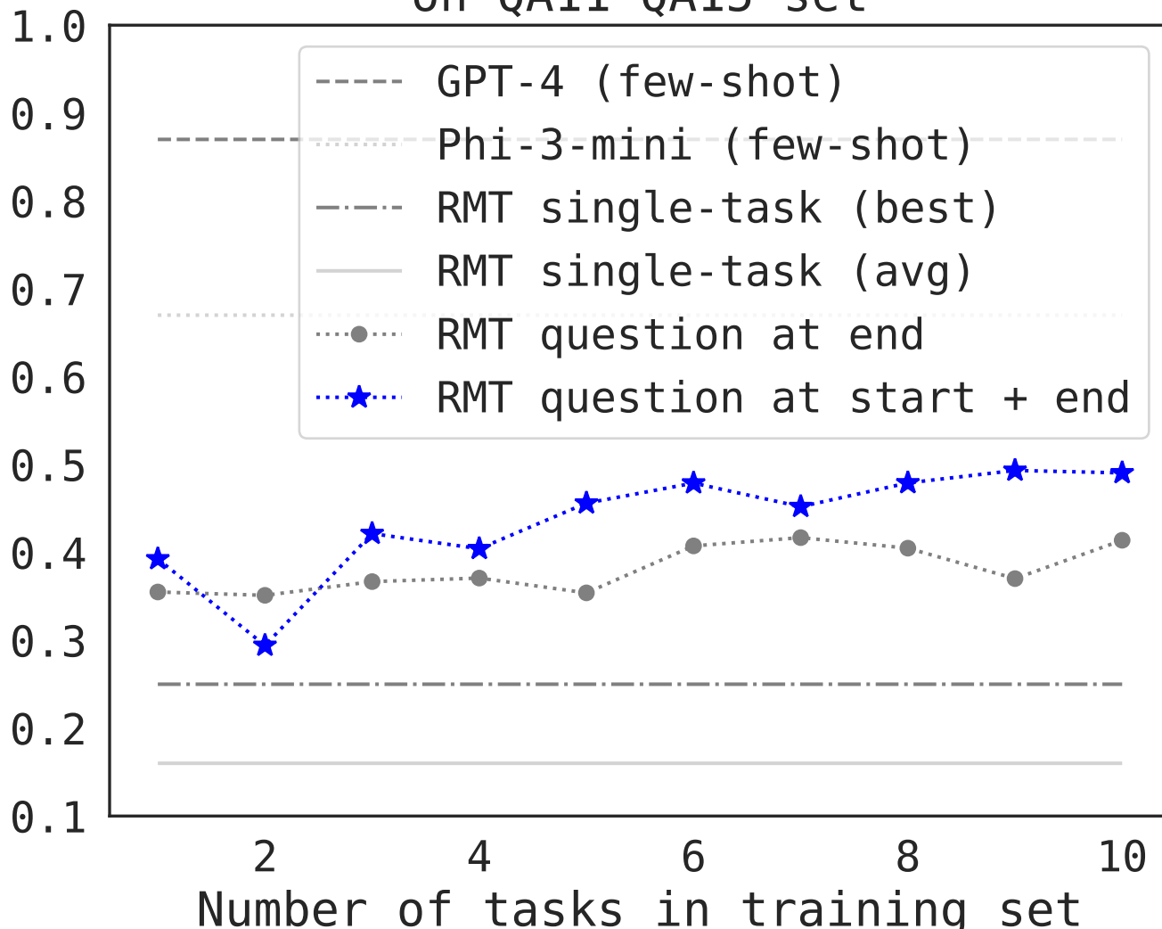
Average performance on QA11-QA15 set
